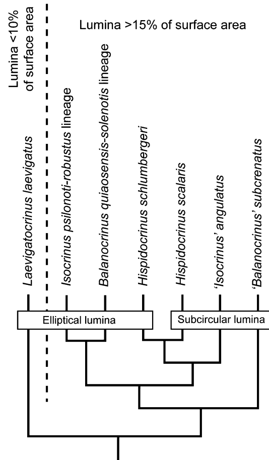
Fig. 4 Cladogram showing relationship between various Late Triassic and Early Jurassic crinoid species and species groups, as inferred from the shape and area of stereom lumina on columnal latera
