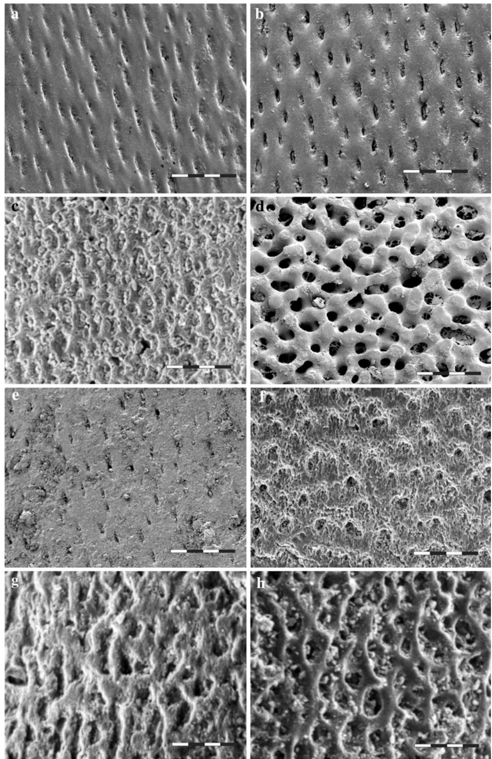
Fig. 2 All figures are of columnal latera unless otherwise indicated. Scale bar 100 \mu\text{m} . a En echelon perforate stereom with elliptical lumina. Endoxocrinus parrae (Gervais). Recent. BELUM K2010.1.2. b En echelon perforate stereom with elliptical lumina. Endoxocrinus prionodes H.L. Clark. Recent. BELUM K2010.2.2.c ?Labyrinthine stereom. Chariacrinus wuerttembergicus (Oppel). Jurassic, Toarcian, Whitby Mudstone Formation, Cleeve Hill, Gloucestershire, England. BM E70412. d Labyrinthine stereom. Democrinus cf. brevis . Recent. BELUM K2010.3.2. e En echelon perforate stereom with very small, widely spaced elliptical lumina. Laevigatocrinus laevigatus (Münster). Triassic, Carnian, Cassian Formation, Cion del Coute, Italy. Muschelkalkmuseum Ingelbongen. f En echelon perforate stereom with weakly elliptical lumina. Balanocrinus subcrenatus (Münster). Triassic, Carnian, Cassian Formation, St Cassian, Italy. BMNH E67484 g. Labyrinthine stereom. Plicatocrinus inornatus Simms. Jurassic, Toarcian, Beacon Limestone Formation, Watton Cliff, Dorset, England. BM E70612. h Labyrinthine stereom. Millerocrinus ? alpinus (Gumbel). Jurassic, Toarcian, Marlstone Rock Formation, Thorncombe Beacon, Dorset, England. BM E70515
