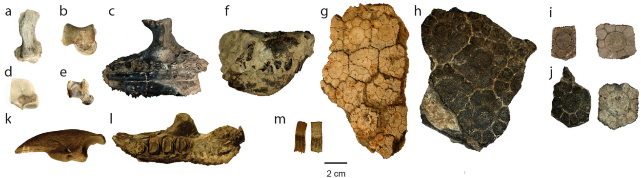
Fig. 2 a Propalaeohoplophorinae indet. (PIMUZ A/V 5593) right calcaneus in ventral view; b Propalaeohoplophorinae indet. (PIMUZ A/V 5594) right astragalus; c Propalaeohoplophorinae indet. (PIMUZ A/V 5590) cranium with mf2–mf7 in palatal view; d Megatherioidea indet. (PIMUZ A/V 5618) right astragalus; e Dasypodidae indet. (PIMUZ A/V 5588) right astragalus (dorsal view); f Peltephilus sp. (PIMUZ A/V 5589), broken skull in right lateral view; g osteoderm of
