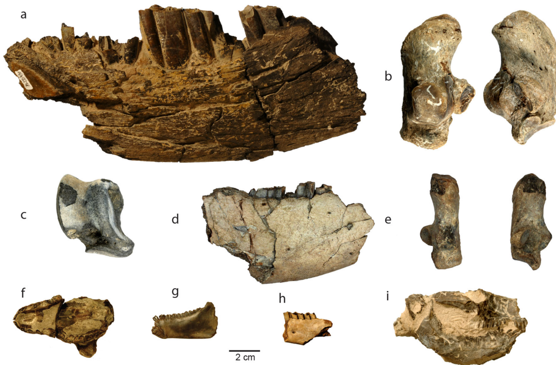
Fig. 5 a Nesodon imbricatus (PIMUZ A/V 5298) left dentary; b Nesodon imbricatus (PIMUZ A/V 5518) right calcaneus in dorsal and medial views; c Nesodon imbricatus (PIMUZ A/V 5517) right astragalus in dorsal view; d Adinotherium sp. (PIMUZ A/V 5483) right dentary; e Adinotherium sp. (PIMUZ A/V 5466) left calcaneus
